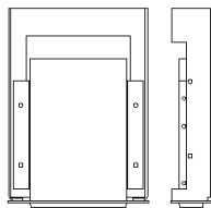
505-335 3 1/2 FLOPPY DRIVE ADAPTER FITS 25MM (1") HIGH DRIVES
