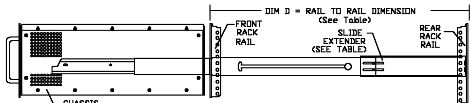
CHASSIS (Shown in extended position)
